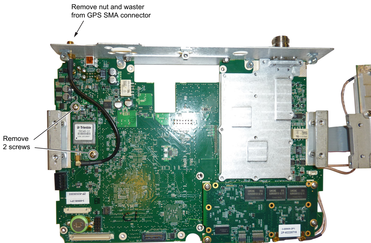
Figure 6-8. Removing the GPS PCB from the Motherboard (SPA PCB already removed)
